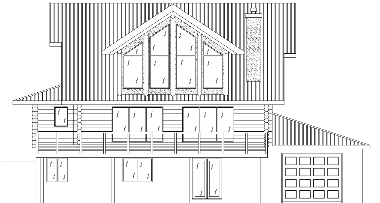
—FRONT ELEVATION—
